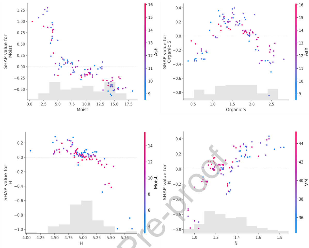
Fig. 2. SHAP feature dependence scatter plots for the XGBoost model to show the complexity of relationships between coal parameters.
