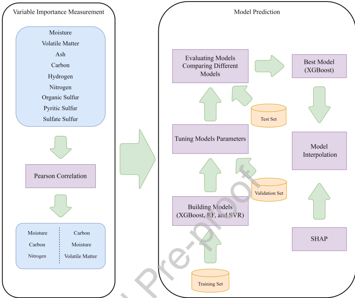
Fig. 1. Modeling sequence for coking coal indexes.
